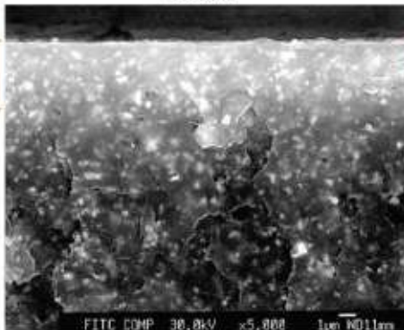
Penetration of coating: 5-10 micron* Different material for different layer
