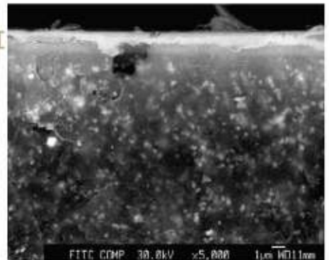
Penetration of coating: 1 micron* Single material applied multiple times
